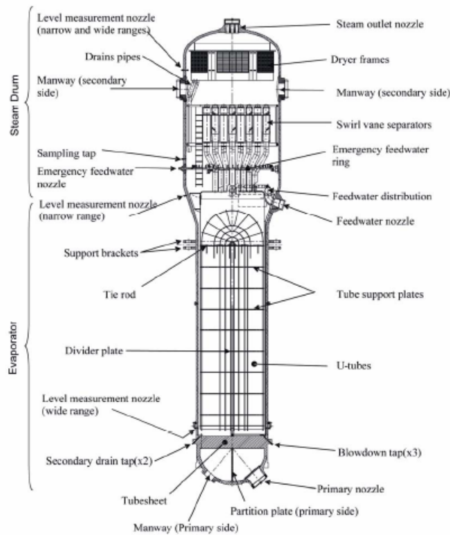
Figure 5 – Steam Generator
